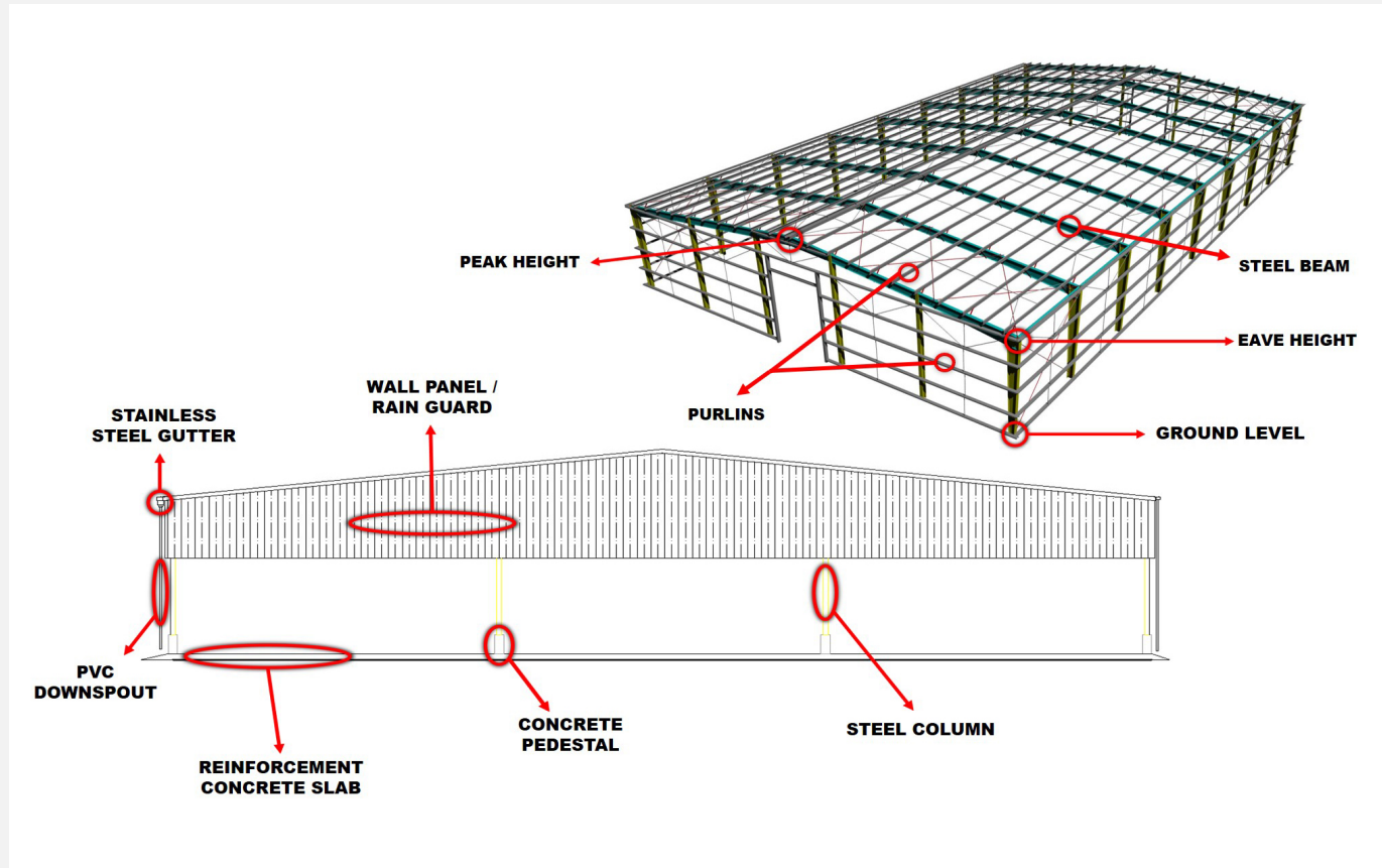
Warehouse Building System
